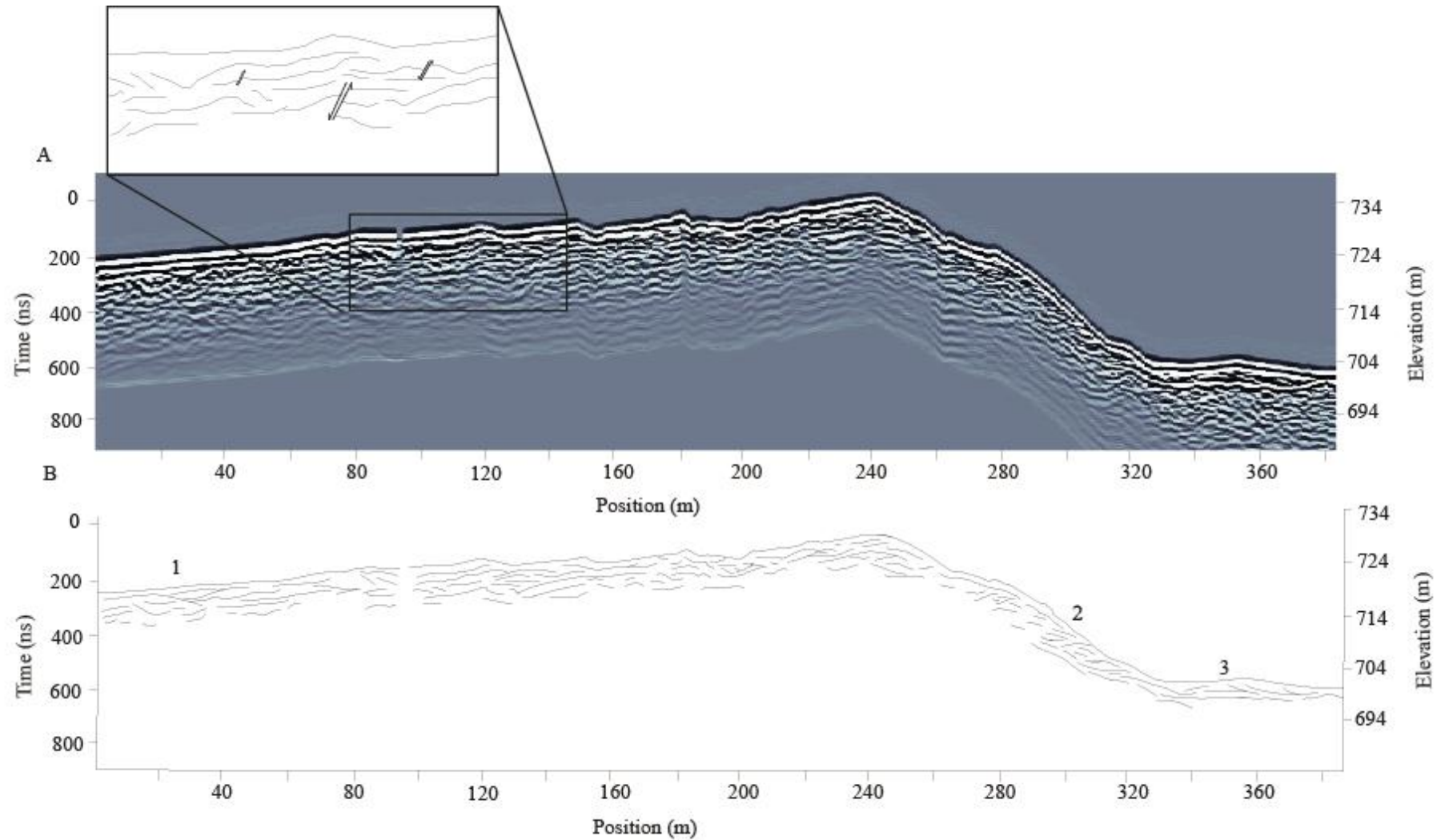
Figure 4.17: A) GPR data from profile T2, showing the internal structure of the subdued terminal moraine B) interpretation diagram for the profile T2 showing 1) sub-parallel reflections interpreted as the ice distal slope of an ice contact fan; 2) steeply up-glacier dipping reflections interpreted as rectilinear slopes ; and 3) strong reflection interpreted as a sedimentary surface. The shadow which is shown along the entire profile, underneath the reflection is an artefact and is not interpreted as part of this profile. Insert box showing increased sinuosity of the reflections and a number of faults.
